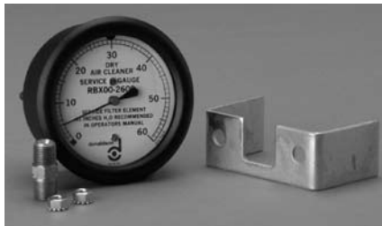
Gauge Part No. X002700 Restriction Limit: 60" H 2 O/ 15 kPa Kit includes restriction tap fitting (P112257), nuts, mounting bracket and installation instructions.
