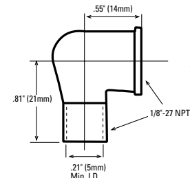
Part No. P105622 • 1/8"-27 threads • 90° elbow with threaded end
