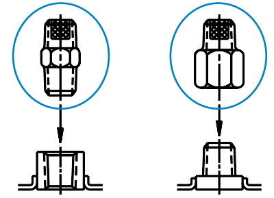
Part No. P100089 • Male threads both ends • 1/8"-27 thread • 0.44" (11mm) hex nut • Internal sintered bronze safety filter
