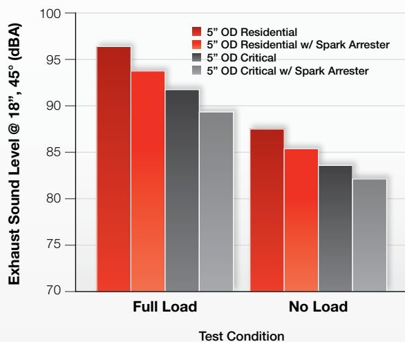
Muffler Comparison on 25 HP V-Twin Engine
