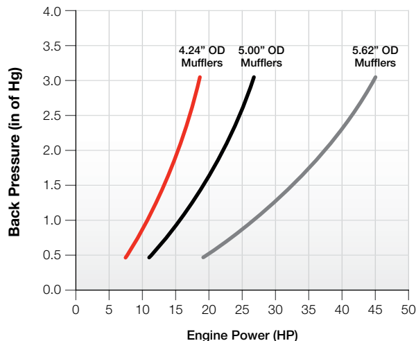
Muffler Selection Chart
